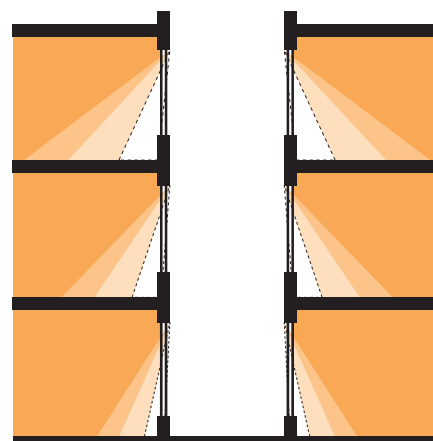
Light well with indicative daylight access shown
