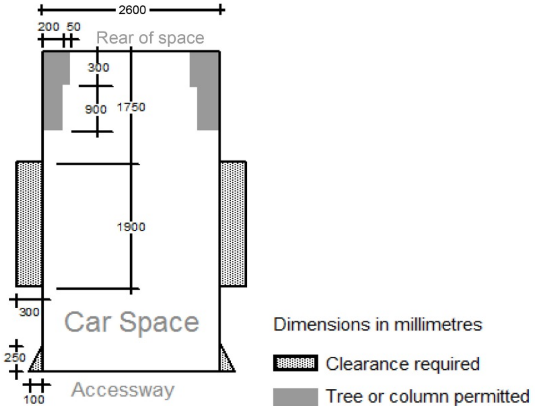
Diagram 1 Clearance to car parking spaces
